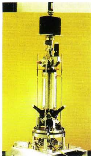
Figure 11. The microgravity clock prototype. The left part is the 60\text{ cm} \times 60\text{ cm} \times 15\text{ cm} optical bench containing the diode laser sources and the various optical components. The right part is the clock itself (about one meter long) containing the optical molasses, the microwave cavity and the detection region.
